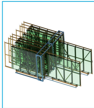
抽屉式仓储架 Drawer type storage rack
