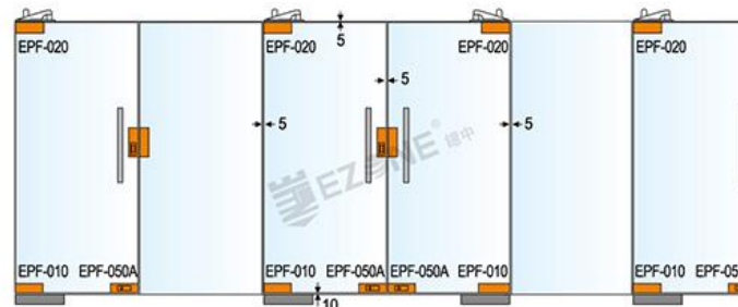
方型门夹扇式样 Square patch fitting models
