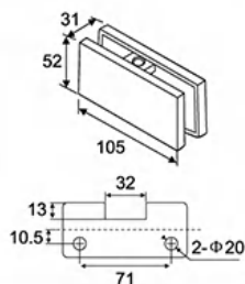
EPF-716 一字夹 Connector for 2 glass panels with screw
