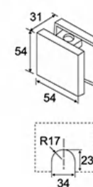
EPF-640 小夹 Connector for glass panel
