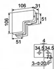
EPF-705B 七字夹 Connector patch with stop
