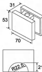
EPF-715 小夹 Connector for glass panel
