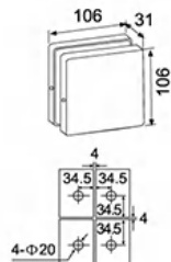
EPF-713 四方夹 Connector for 4 glass panels
