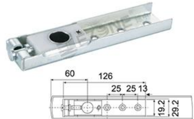
AC-04(下) 枢轴底座: Pivot Bottom Seat
