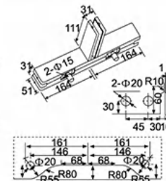
EPF-719 异形夹 Overpanel connector with stop
