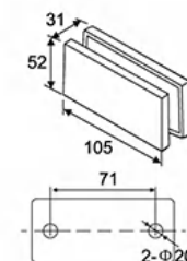
EPF-716B 一字夹 Connector for 2 glass
