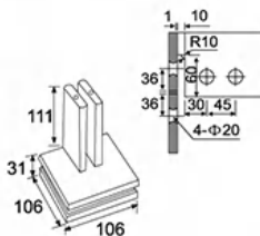
EPF-713 四方夹 Connector for 4 glass panels
