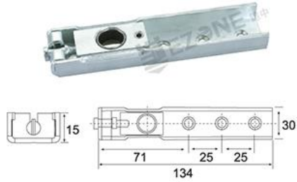
AC-01(下) 枢轴底座: Pivot Bottom Seat
