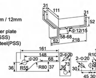
EPF-710 T字夹 Double patch with fin T
