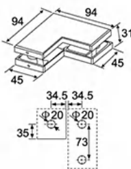
EPF-705B 七字夹 Connector patch with stop
