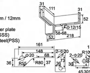
EPF-709R 右夹 Overpanel "R" patch with fin
