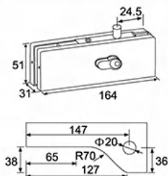
EPF-704 异形夹 Connector patch
