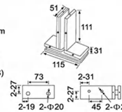
EPF-719 异形夹 Overpanel connector with stop
