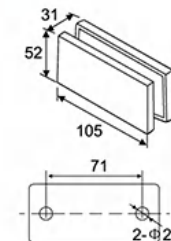
EPF-716A 一字夹 Connector for 2 glass
