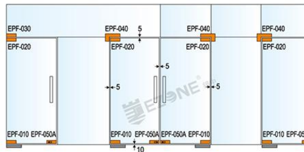
异型门夹扇式样 Irregular patch fitting models
