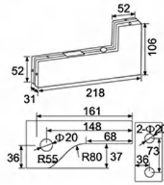
EPF-040B 副曲夹 Overpanel strike box "L" patch
