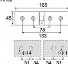
ESH-1076 45# 弧面外开单边 45# Outer opening single-sided
