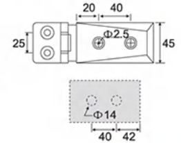
ESH-1067 菱形外开双边 Outer opening bilateral
