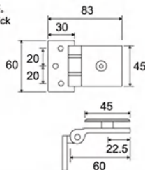
ESH-1089 斜边单边 Oblique single-sided
