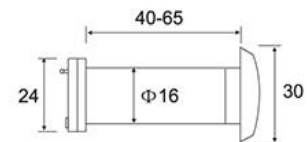
EWD-3035 200° 猫眼 200° Door viewer
