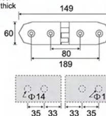
ESH-1073 钝角外开双边 Obtuse Angle Outer opening Double
