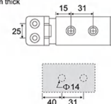
ESH-1077 45# 平面外开单边 45# Out-of plane single-sided
