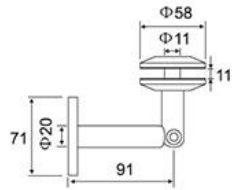
ESD-654 单杆固定杆/连接墙体 Wall to glass connector STD(cable connection)
