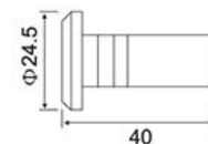
EWD-3038 插销防尘套 Dust cover
