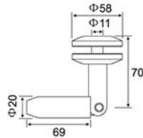
ESD-656 吊索固定杆/与玻璃连接 Front cantilever glass bracket STD(cable connection) (再大玻璃承重100kg) The maximum weight is 100kg
