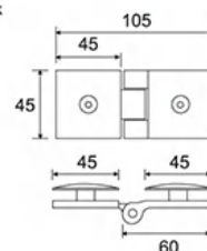
ESH-1092 弧面双边 Camber bilateral
