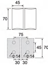
ESH-1064 70# 弧面外开单边 70# Outer opening single-sided
