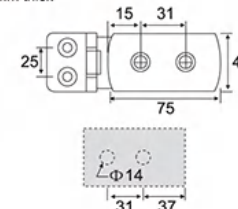
ESH-1075 45# 弧面外开双边 45# Outer opening bilateral
