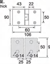
ESH-1053 90# 外开双边 90# Outer opening bilateral
