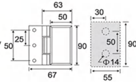
ESH-1055 90# 斜边内开双边 90# Inside opening bilateral
