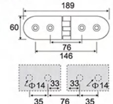
ESH-1069 弧面外开双边 Outer opening bilateral
