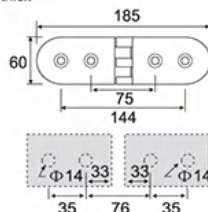
ESH-1072 钝角外开单边 Obtuse Angle Outer opening sided
