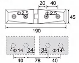
ESH-1068 弧面外开单边 Outer opening single-sided
