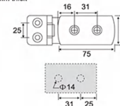
ESH-1077 45# 平面外开单边 45# Out-of plane single-sided
