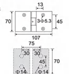
ESH-1061 斜面外开双边 Outside opening bilateral
