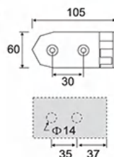
ESH-1073 钝角外开双边 Obtuse Angle Outer opening Double
