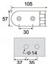
ESH-1071 弧边外开双边 Outer opening bilateral
