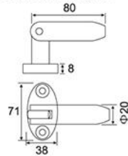
ESD-656 吊索固定杆/与玻璃连接 Front cantilever glass bracket STD(cable connection) (再大玻璃承重100kg) The maximum weight is 100kg
