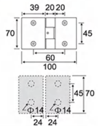
ESH-1060 斜面外开单边 Outside opening single-sided
