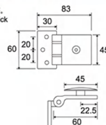
ESH-1091 弧面单边 Camber single-sided
