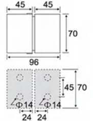
ESH-1059 70# 外开双边 70# Outer opening bilateral
