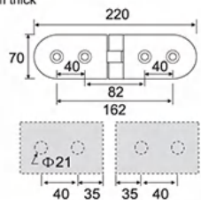
ESH-1048 45# 圆角外开单边 45# Rounded corners outer opening single-sided
