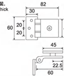
ESH-1093 直边单边 Straight single-sided
