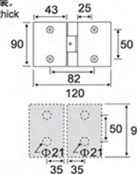
ESH-1052 90# 外开单边 90# Outer opening single-sided
