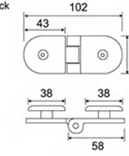
ESH-1096 圆珠双边 Round bead bilateral
