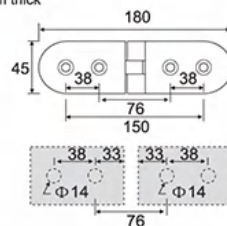
ESH-1049 45# 圆角外开双边 45# Rounded corners outer opening bilateral
