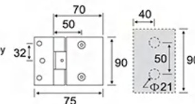
ESH-1051 圆角外开双边 Rounded corners outer opening bilateral
