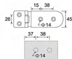
ESH-1049 45# 圆角外开双边 45# Rounded corners outer opening bilateral
