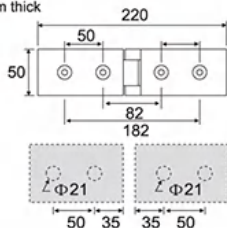
ESH-1047 长圆外开双边 Long round outward opening bilateral
