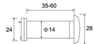
EWD-3037 200° 猫眼 200° Door viewer
