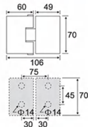
ESH-1065 70# 弧面外开双边 70# Outer opening bilateral
