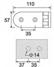
ESH-1069 弧面外开双边 Outer opening bilateral
