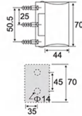
ESH-1063 70# 外开双边 70# Outer opening bilateral
