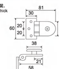
ESH-1095 圆珠单边 Round bead single-sided
