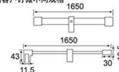
EBA-1118 玻璃固定拉杆 Glass fastness kningthead
