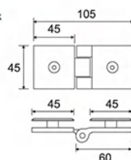
ESH-1090 斜边双边 Oblique bilateral
