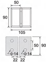
ESH-1055 90# 斜边内开双边 90# Inside opening bilateral
