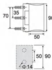
ESH-1057 90# 内开弧面双边 90# Outer opening bilateral
