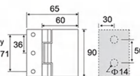
ESH-1053 90# 外开双边 90# Outer opening bilateral
