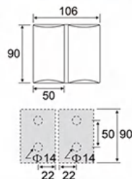
ESH-1057 90# 内开弧面双边 90# Outer opening bilateral
