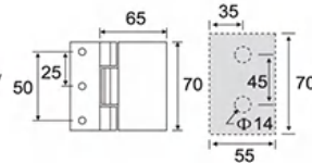
ESH-1065 70# 弧面外开双边 70# Outer opening bilateral
