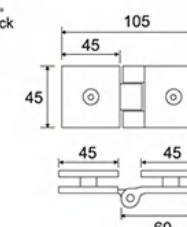
ESH-1094 直边双边 Straight bilateral
